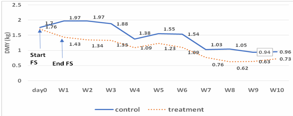
Fig. 2. Daily milk yield (kg) of Barki does with one week feed shortage.
